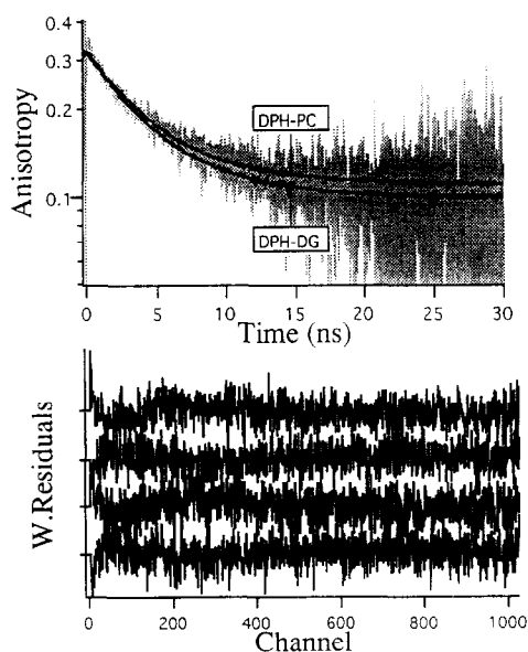
Fig. 1. Experimental and fitted anisotropy decays of DPH-DG and DPH-PC in DOPC vesicles. The smooth curve corresponds to the optimal fit with the r_{g3} model assuming a Gaussian orientation distribution. In the lower panel the weighted residuals of the fit to the perpendicular and parallel decay curves of DPH-PC (upper two curves) and DPH-DG (lower two curves) are presented.
