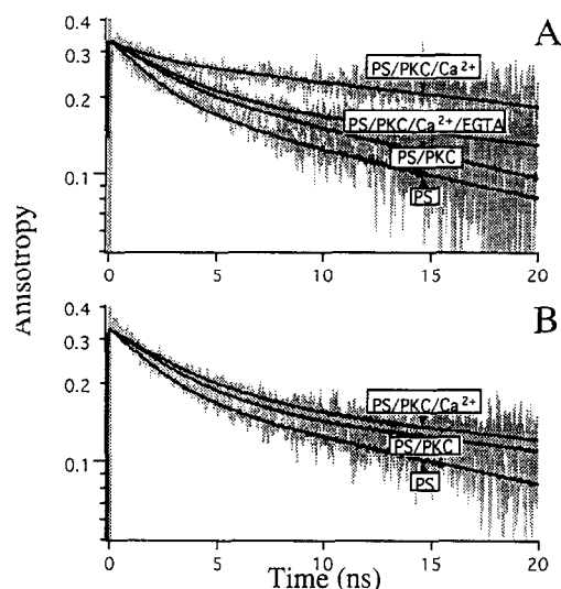
Fig. 4. Experimental anisotropy decays of DPH-DG (A) and DPH-PC (B) in thesitt micelles containing 10 mole% PS at various binding conditions (see text).
