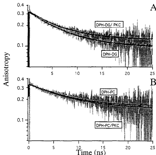
Fig. 2. Experimental anisotropy decays of DPH-DG (A) and DPH-PC (B) in vesicles of DOPC/PS (80:20) in the presence and absence of PKC (0.4 \mu M). In the blank experiments without PKC, the dialysis buffer of PKC was added to the vesicles. The smooth curve corresponds to the optimal fit with the r_{g3} model assuming a Gaussian orientation distribution.
