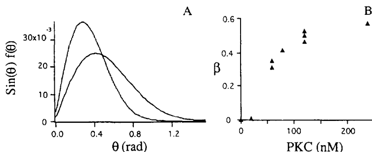
Fig. 3. (A) Orientation distributions of probe molecules with Gaussian width of 0.65 (—) and 0.41 (---). These values correspond to the optimised values of free and PKC-bound DPH-DG, respectively. (B) The fractional contribution ( \beta ) of bound DPH-DG with Gaussian width \theta_{gb} as a function of PKC concentration. The orientation distribution of DPH-DG was assumed to be composed of two Gaussian distributions of free and bound DPH-DG as described in the Experimental procedures. In this analysis the motional freedom of the free DPH-DG lipids \theta_{gf} was fixed to the value obtained in the absence of PKC. The total lipid concentration was 15 \mu M .
