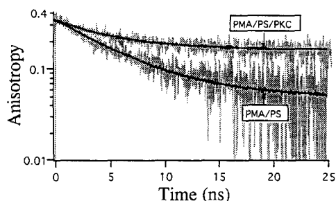
Fig. 5. Anisotropy decays of dansyl-PMA in mixed micelles in the presence and absence of PKC. The micelles were composed of this, 10 mole% PS. The smooth curve through the data points represents an optimised fit with a model consisting of a sum of three exponentials.
